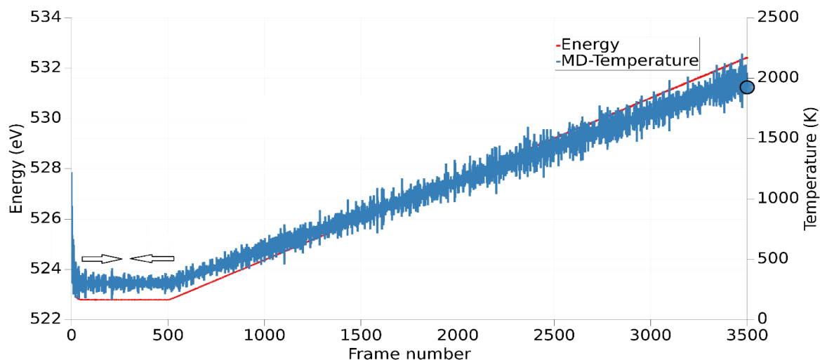
Figure 4. Values of total energy and temperature of the \text{La}_4\text{Mn}_2\text{InGe}_4 compound taken every 100 (25 fs) MD steps.
